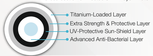
Cross-section of "Vectus Silk 4 Layer" water tank
