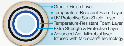
Cross-section of "Vectus Granito 6 Layer" water tank
