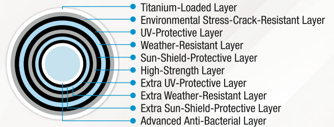
Cross-section of "Vectus Horizontal" water tank
